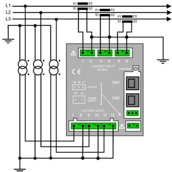
Medium/High Voltage 3 PTs 3 CTs Configuration 3P 4W
